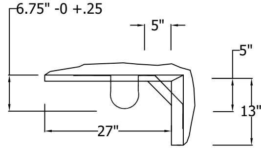
TOP VIEW LEFT OUSIDE CORNER
