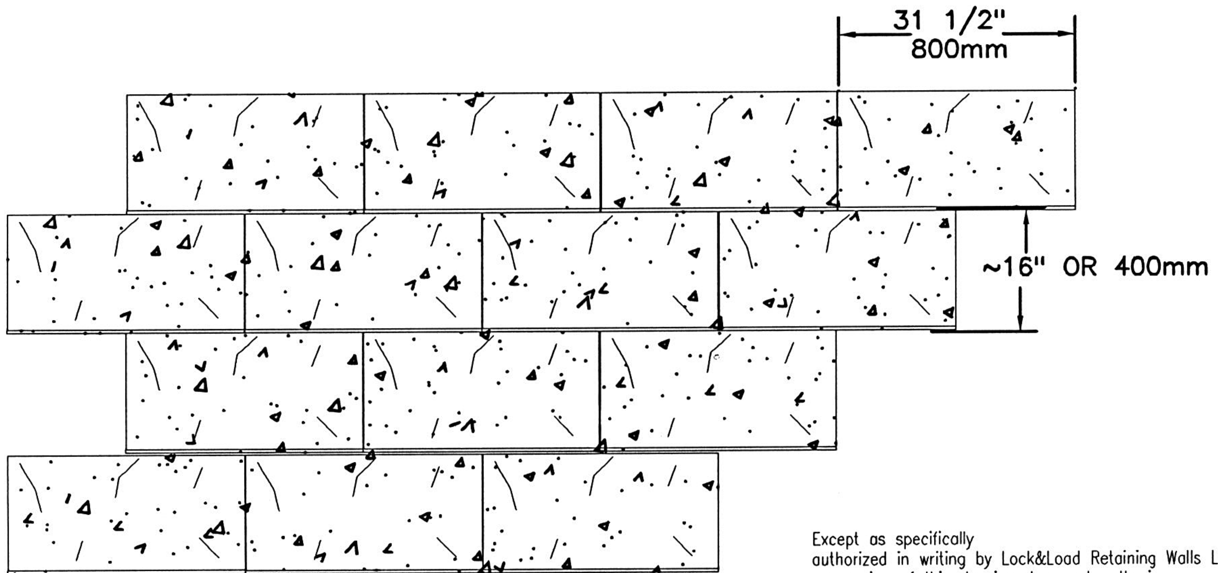
TYPICAL ELEVATION
